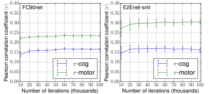
Figure 5: The effect of the number of training iterations on correlations between predicted and ground truth outcome scores (on test data) for FC90net ( left ) and E2Enet-sml ( right ) architectures. The standard deviation of each of the five randomly initialized models is shown at each 10K iterations as vertical error bars.
