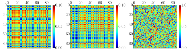
Figure 4: (Left and center) Sample diffuse whole brain injury patterns. (Right) Sample diffuse injury synthetic connectome with two diffuse injury patterns and noise applied.
