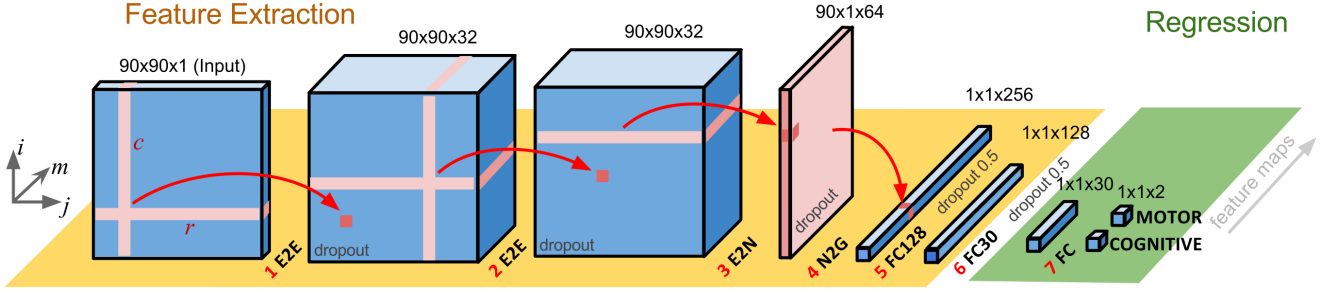
Figure 1: Schematic representation of the BrainNetCNN architecture. Each block represents the input and/or output of the numbered filter layers. The 3rd dimension of each block (i.e., along vector m ) represents the number of feature maps, M , at that stage. The brain network adjacency matrix (leftmost block) is first convolved with one or more (two in this case) E2E filters which weight edges of adjacent brain regions. The response is convolved with an E2N filter which assigns each brain region a weighted sum of its edges. The N2G assigns a single response based on all the weighted nodes. Finally, fully connected (FC) layers reduce the number of features down to two output score predictions.
